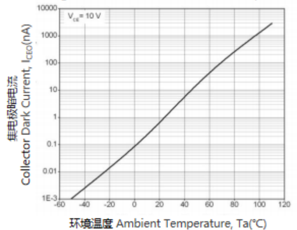
Figure 6. Dark Current vs Ambient Temperature
