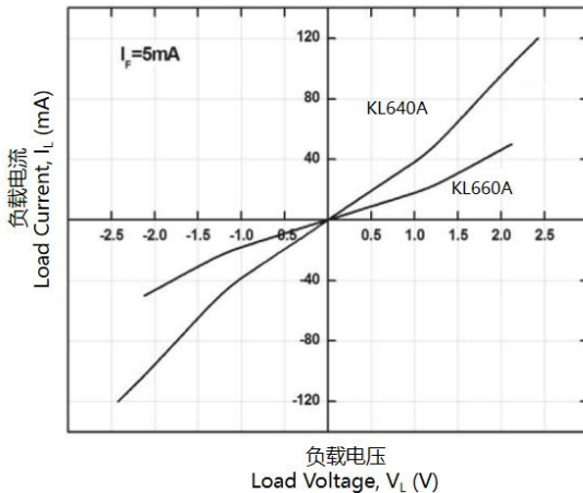
Figure 9-1 Load Current vs Load Voltage
