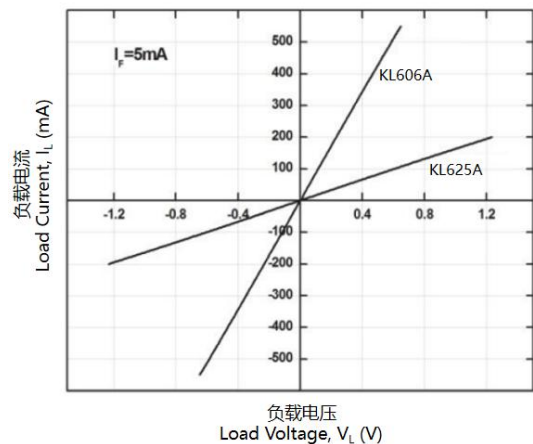
Figure 9-2. Load Current vs Load Voltage
