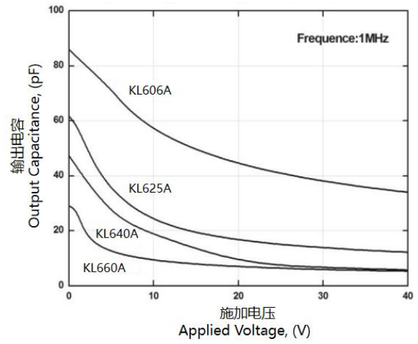
图11. 输出电容 vs 施加电压 Figure 11. Output Capacitance vs Applied Voltage
