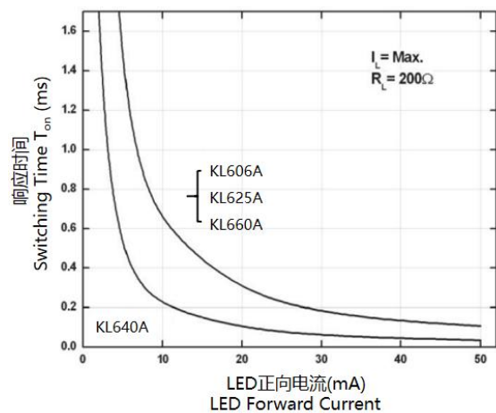
Figure 4-1. Turn-on Time vs LED Forward Current
