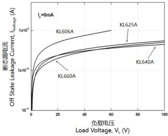
图10. 断态漏电流 vs 负载电压的关系 Figure 10 Off State Leakage Current vs Load Voltage
